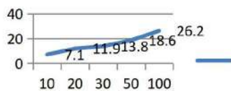
CP300-T20-B1 Compression Ratio and Pressure Curve
